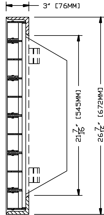
SECTION B - B
