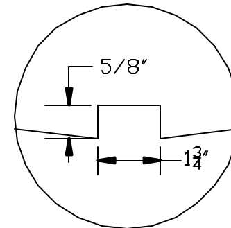
PENETRATING PICKHOLE DETAIL
