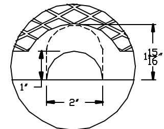
NON-PENETRATING PICKHOLE DETAIL
