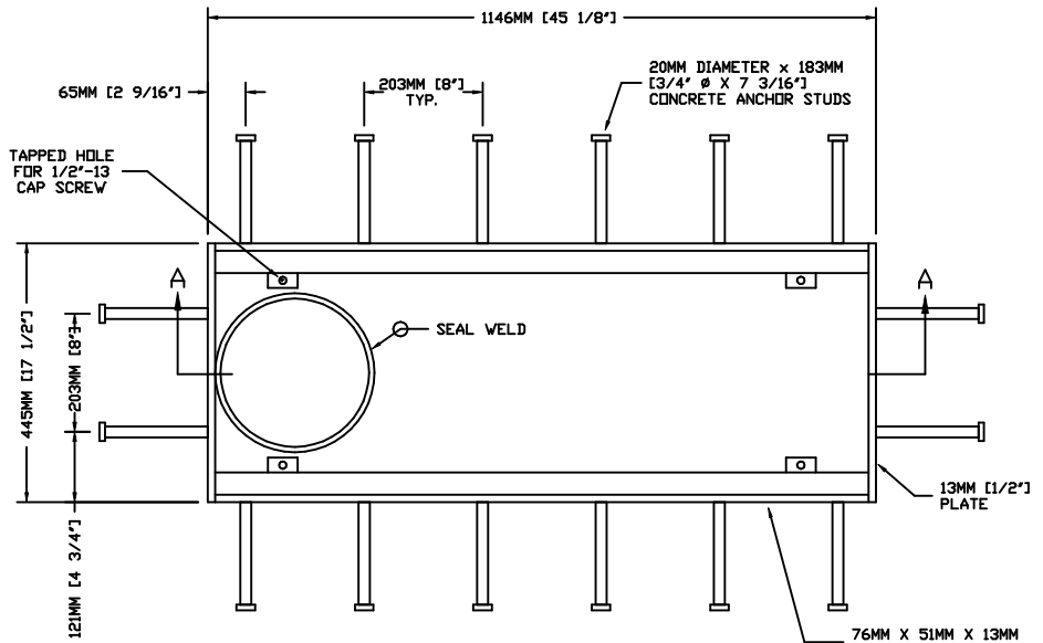
PLAN VIEW
