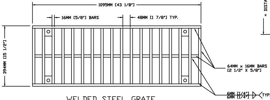
WELDED STEEL GRATE
